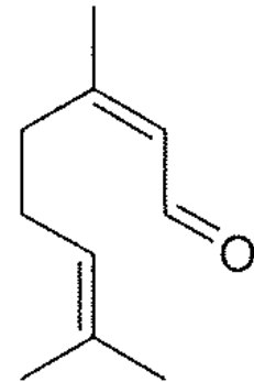
citral
