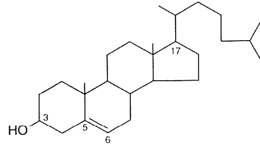
OBR. 15-17. Cholesterol, 3-hydroxy-5,6-cholesten
