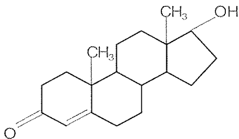
testosteron
